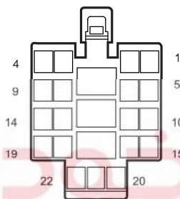
I1_EB Engine W.H. Connector 1 Connecting Body W.H.
