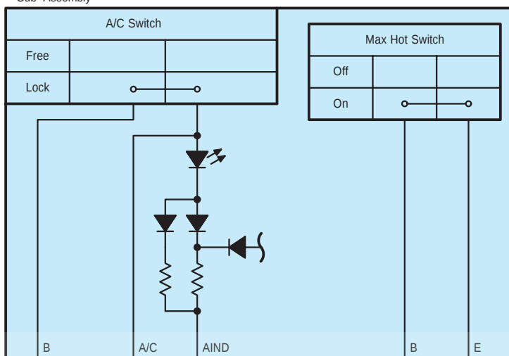
G23 No. 3 Heater Control Sub-Assembly
