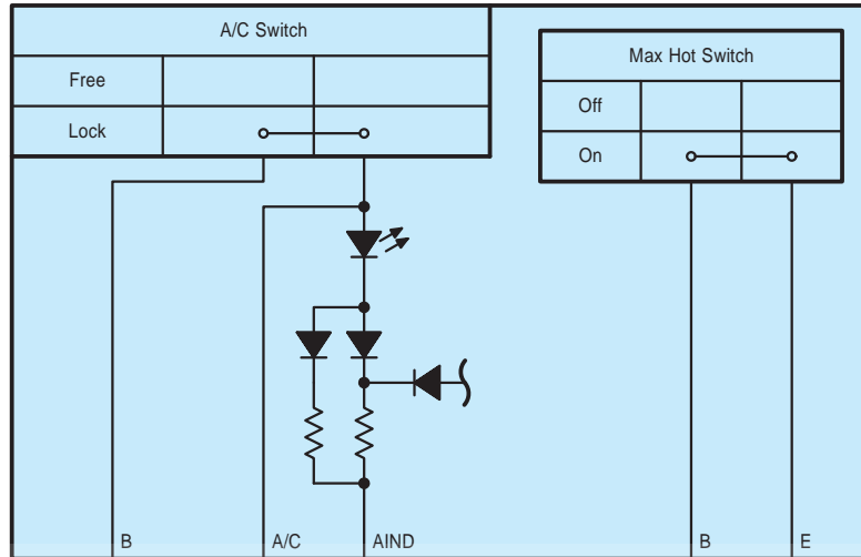
G23 No. 3 Heater Control Sub-Assembly
