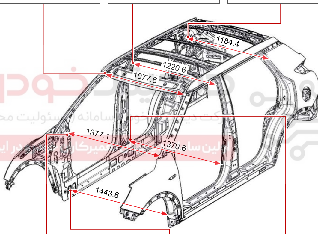
A-pillar inner location hole
