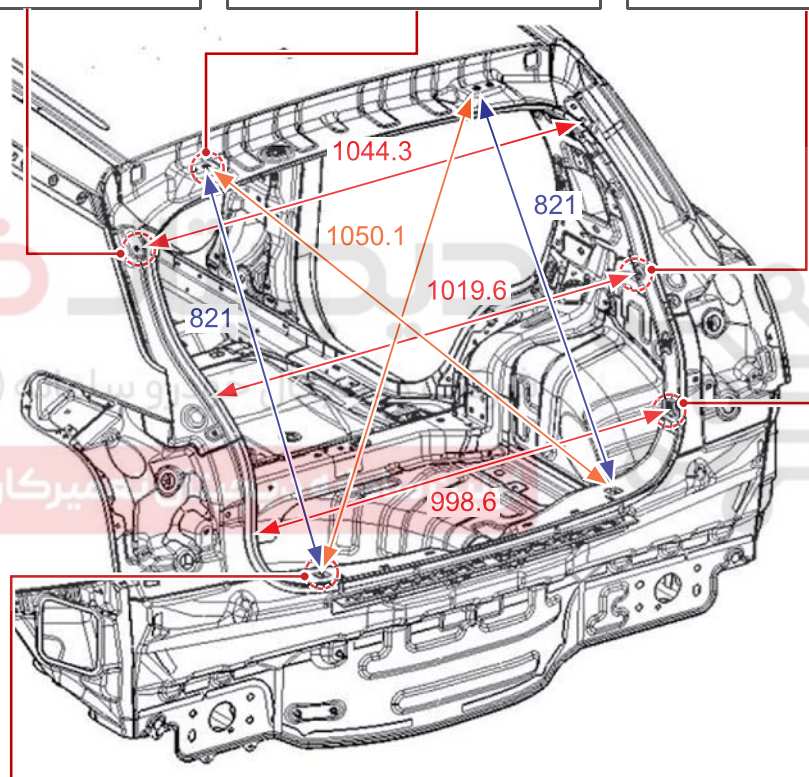
Tailgate glass lift mounting hole
