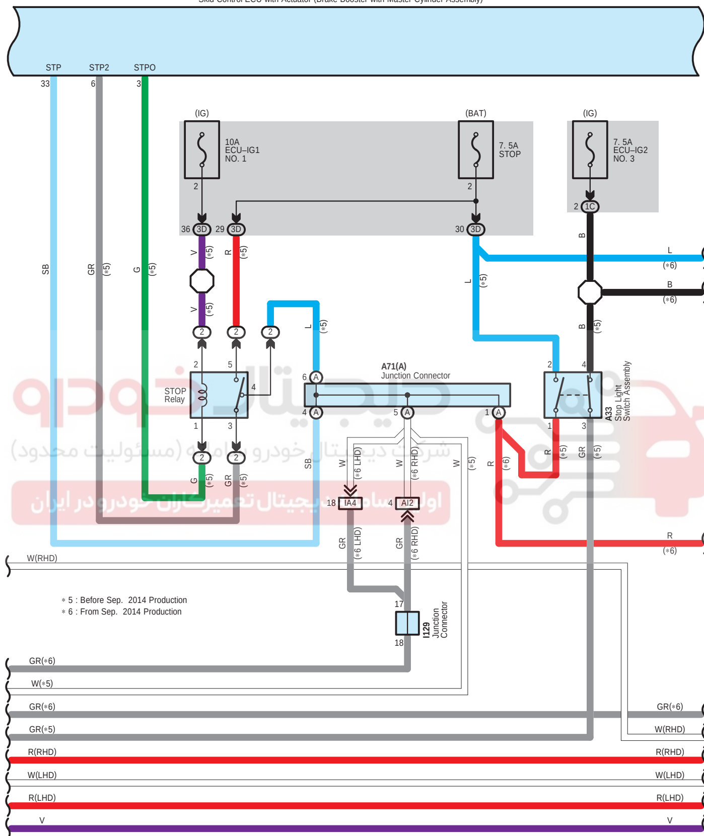
A28 Skid Control ECU with Actuator (Brake Booster with Master Cylinder Assembly)
