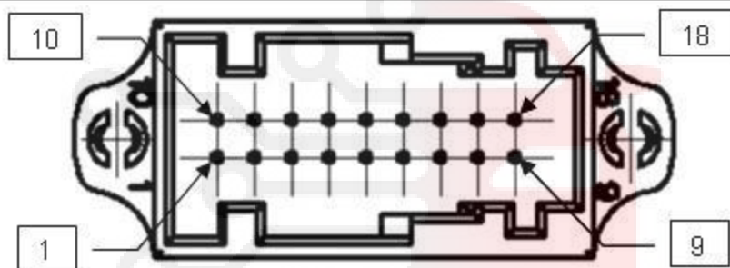
AMP 18PIN VERTICAL CONNECTOR - 953264-1(White)
